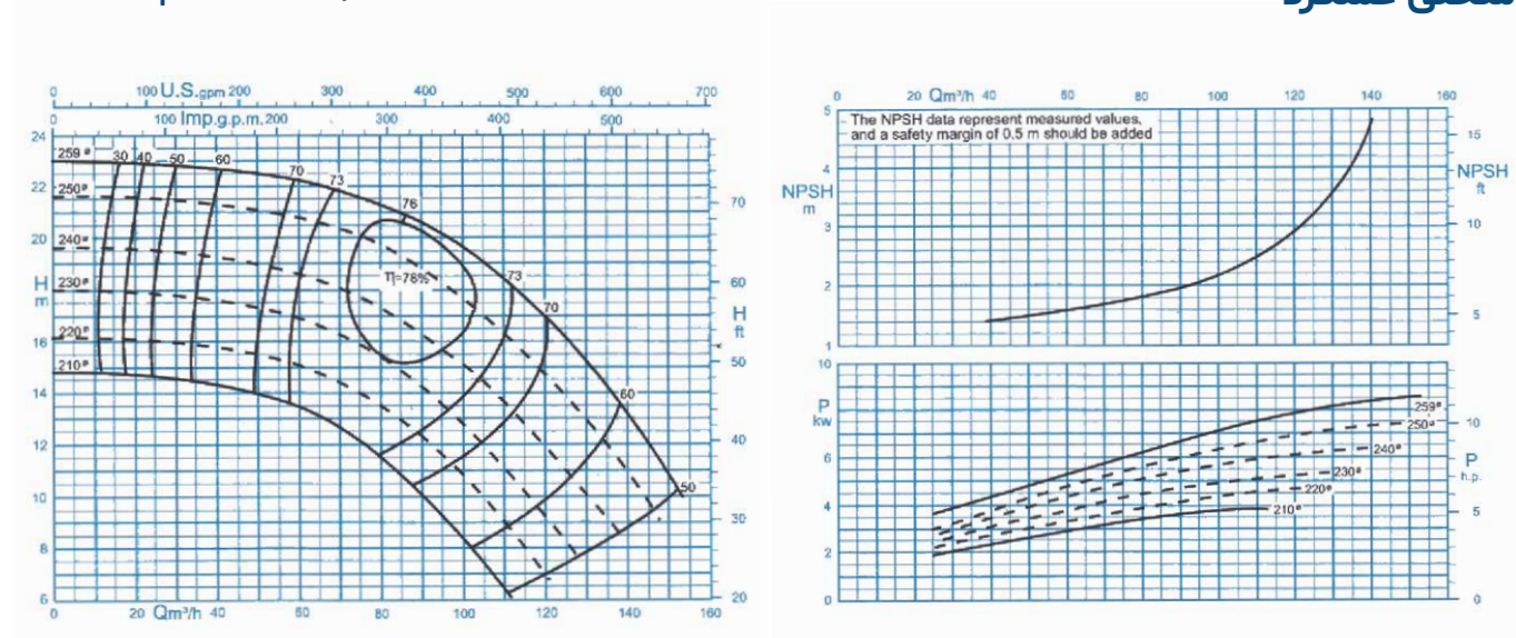
Curves as per Iso 9906/A
